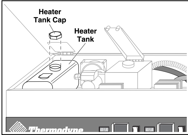
Figure 13: Heater Tank Cap & Reservoir Cap
