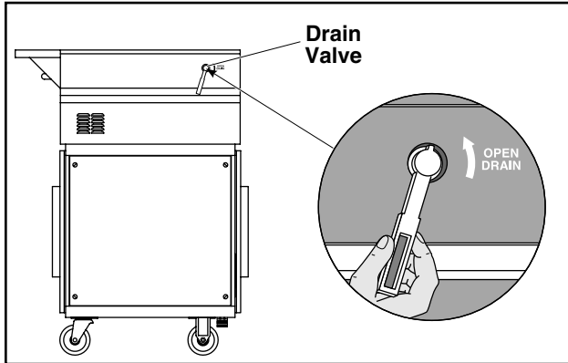
Figure 9: Drain Valve
