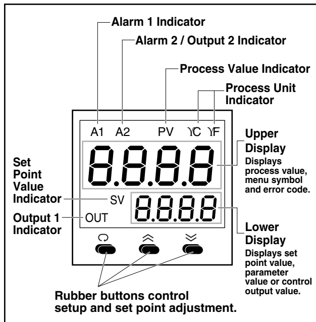
Figure 5: Control Panel Functions
