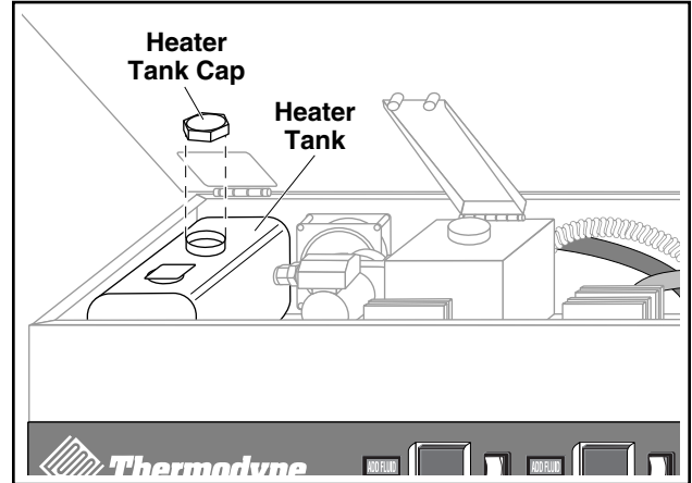
Figure 11: Heater Tank and Cap
