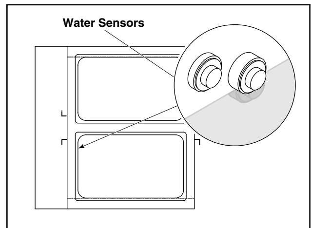
Figure 4: Location of Water Sensors
