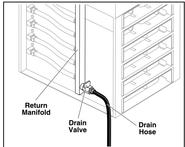
Figure 12: Drain Hose
