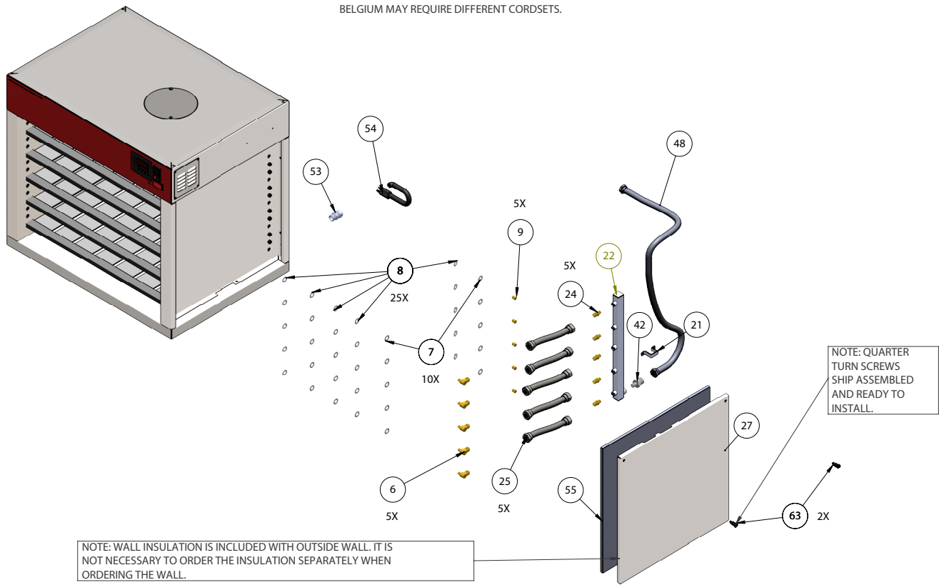
Exploded View 700NDNL - Right Side
