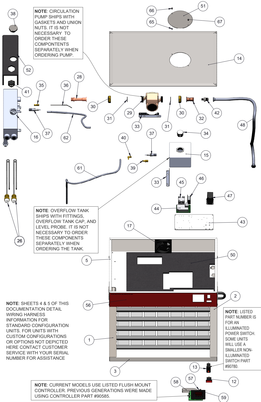
700NDNL PowerHead Exploded View
