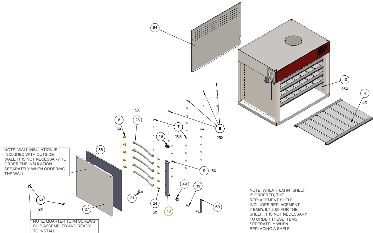
Exploded View 700NDNL - Left Side
