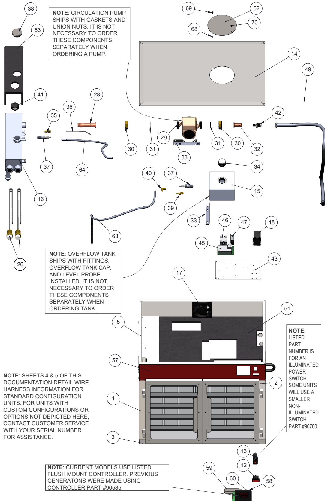
700CT PowerHead Exploded View
