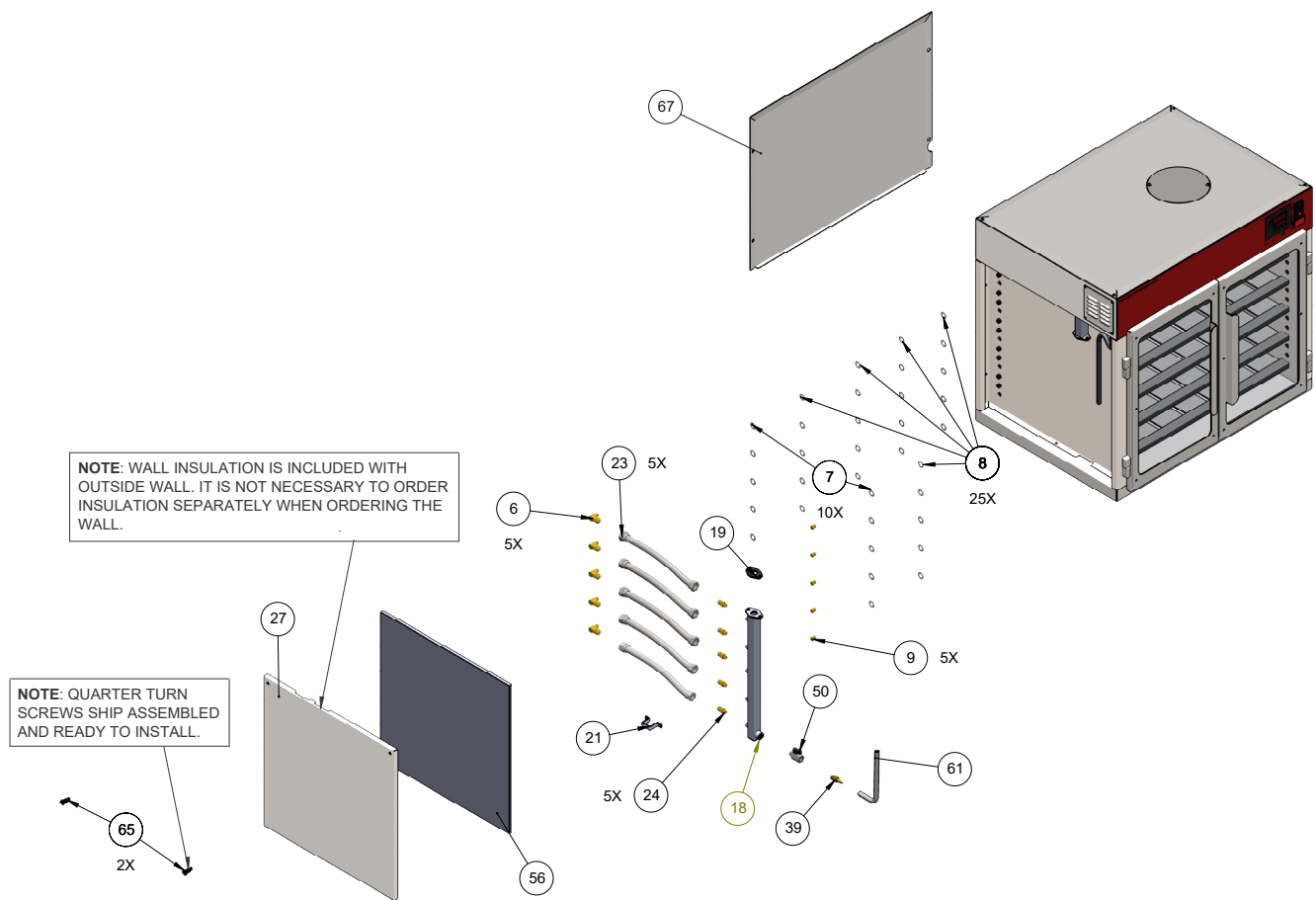
Exploded View 700CT - Left Side
