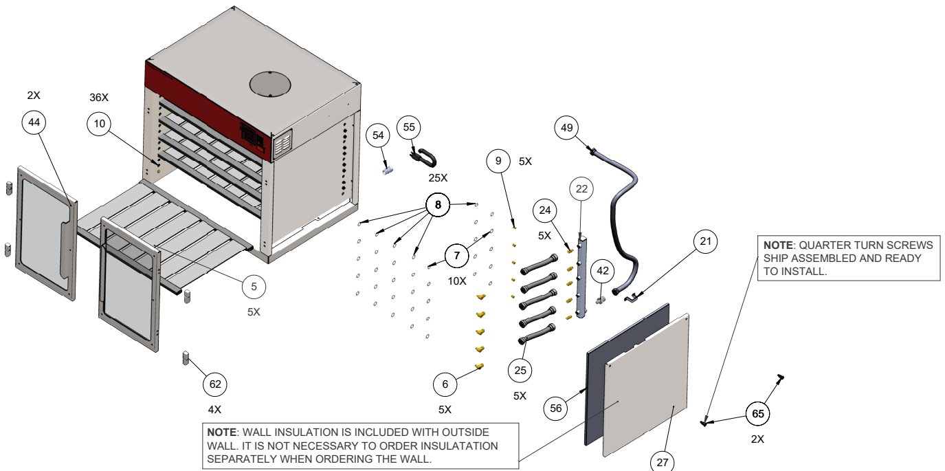
Exploded View 700CT - Right Side
