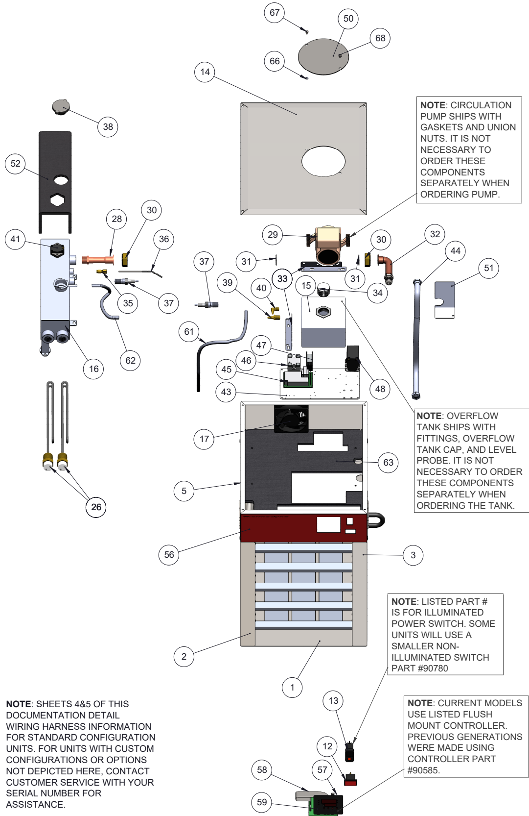
300NDNL PowerHead Exploded View
