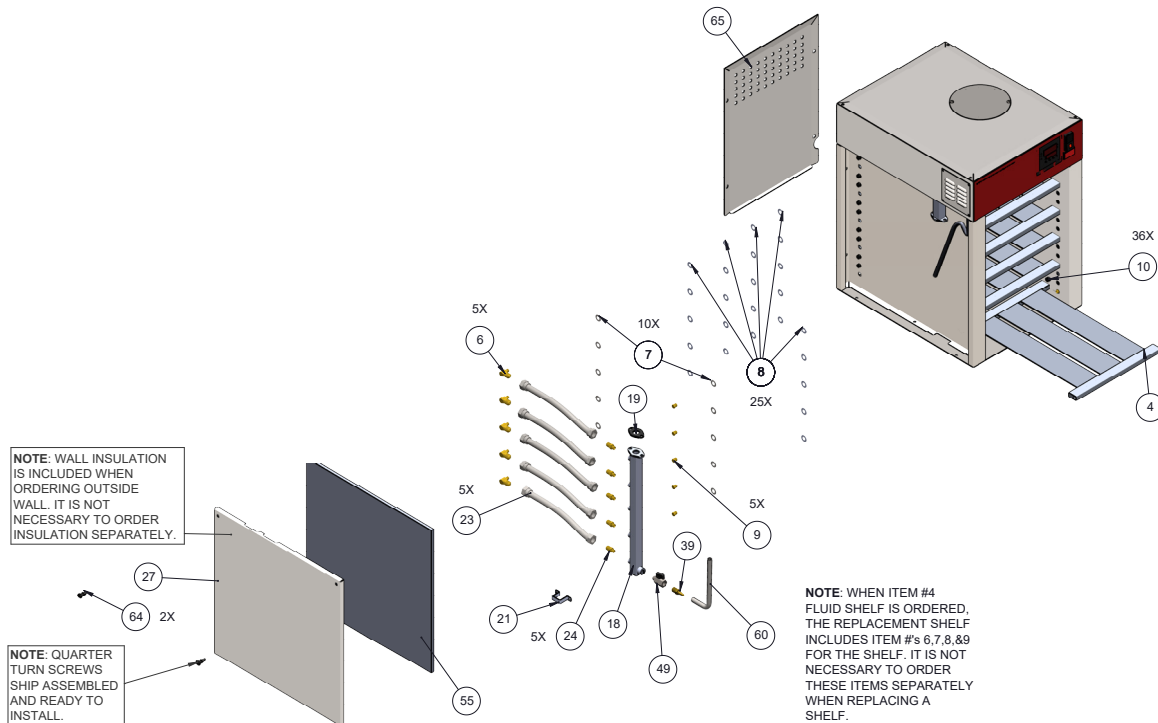
Exploded View 300NDNL - Left Side
