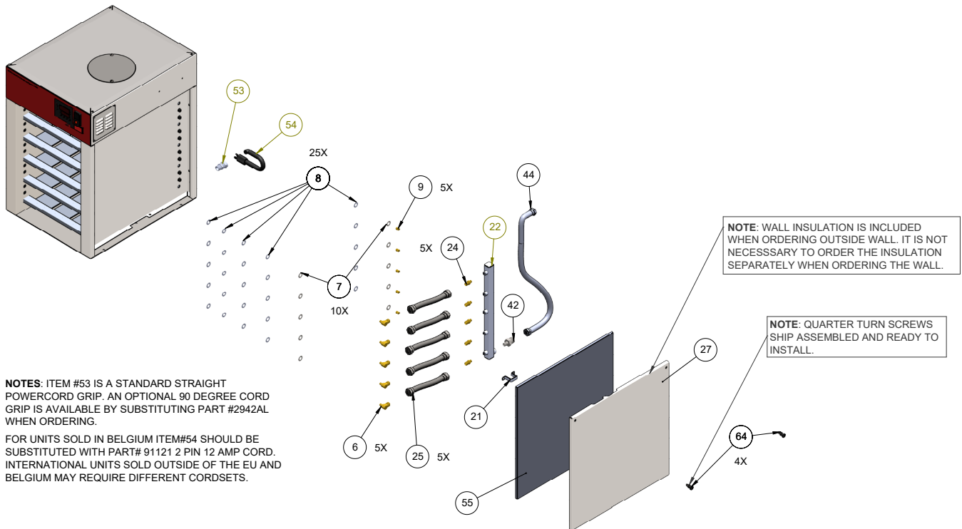
Exploded View 300NDNL - Right Side
