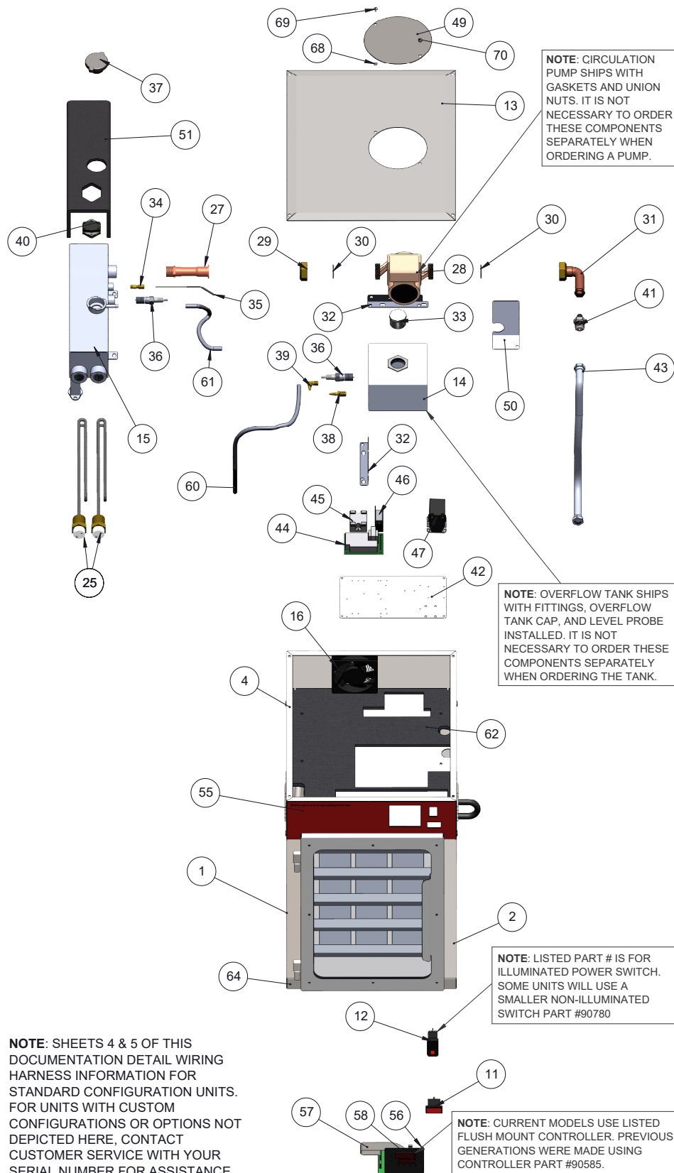
300CT PowerHead Exploded View
