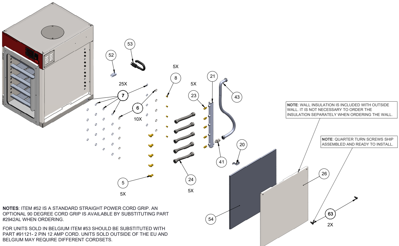
Exploded View 300CT - Right Side
