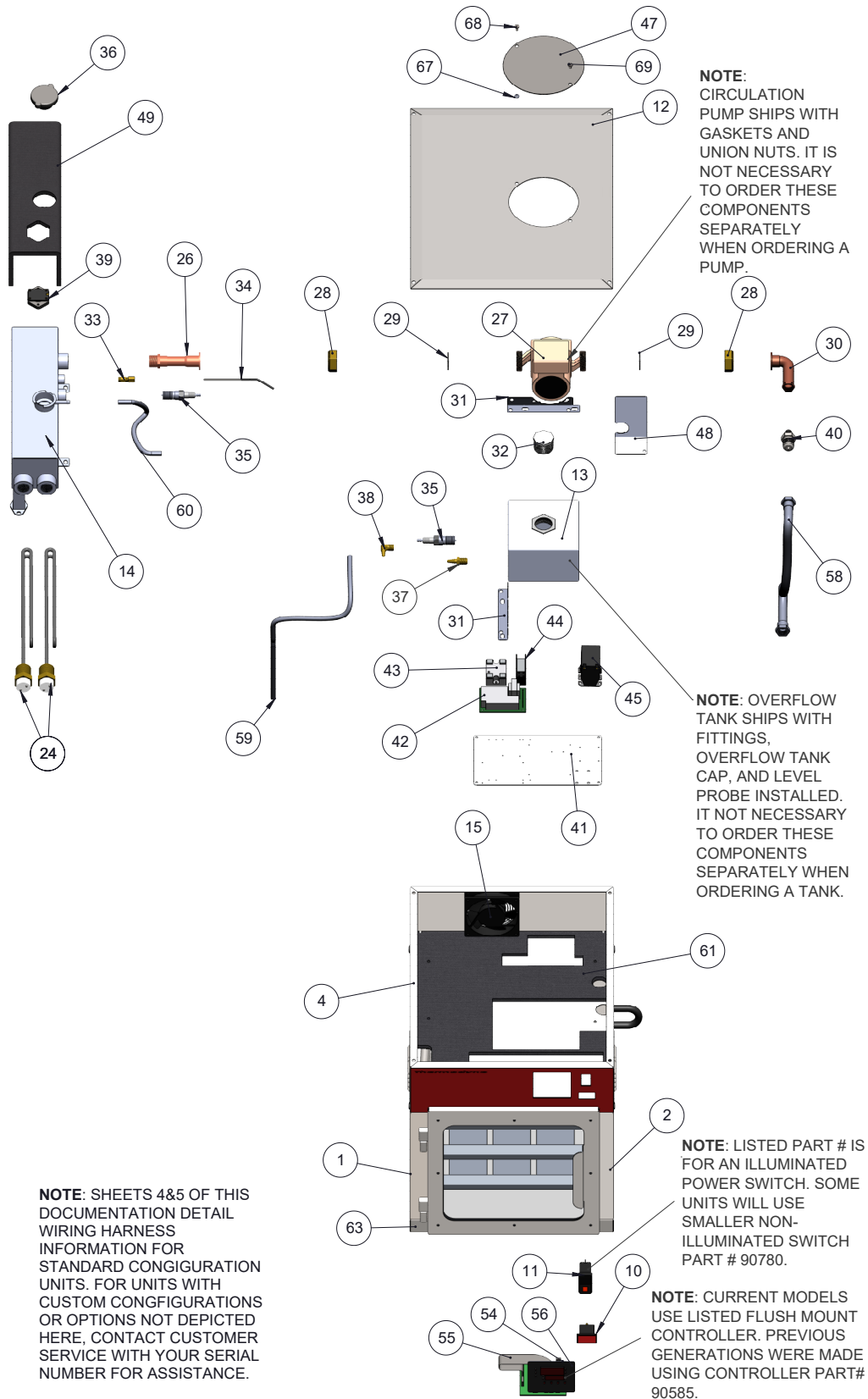
200CT PowerHead Exploded View
