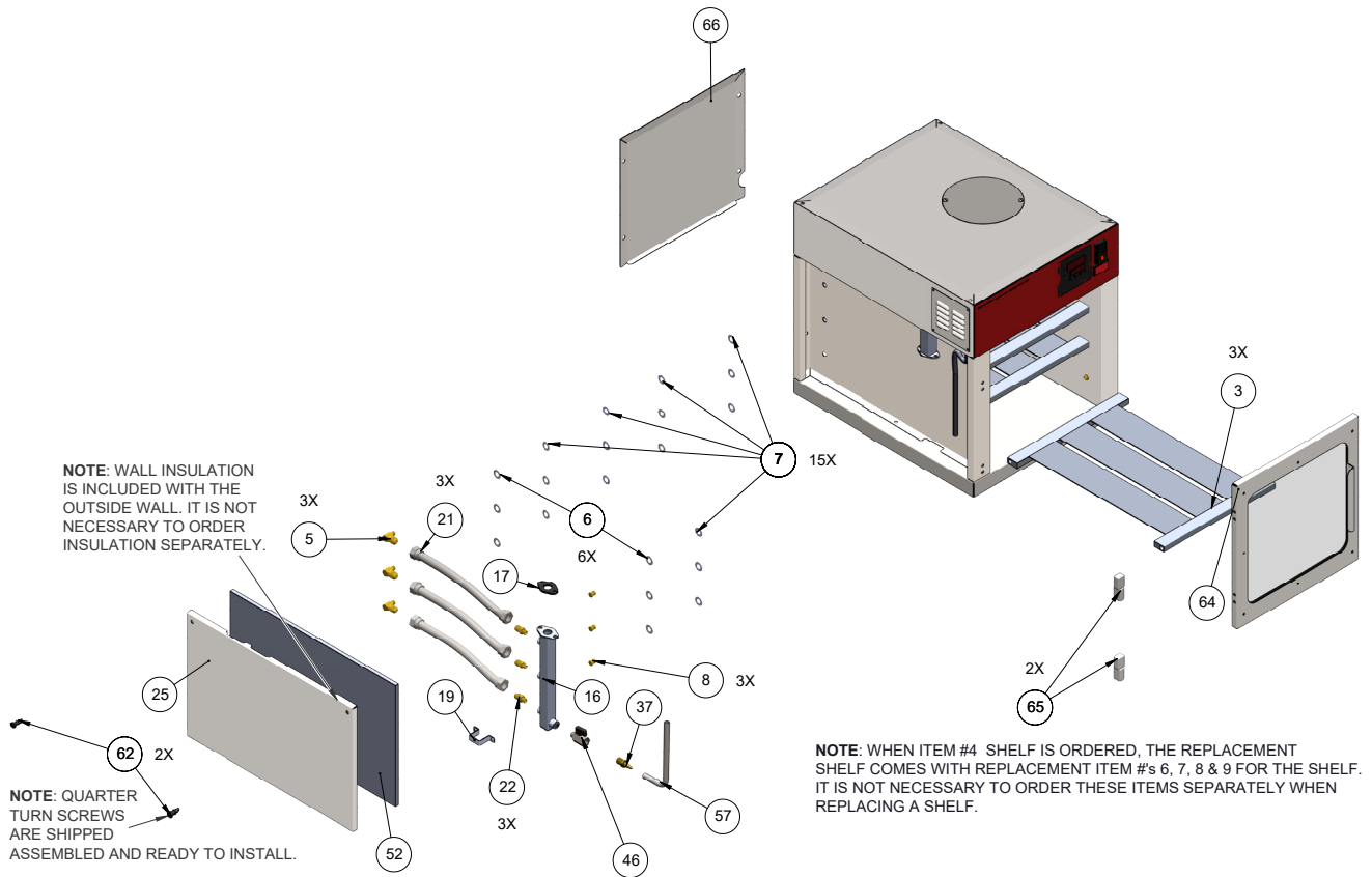
Exploded View 200CT - Left Side
